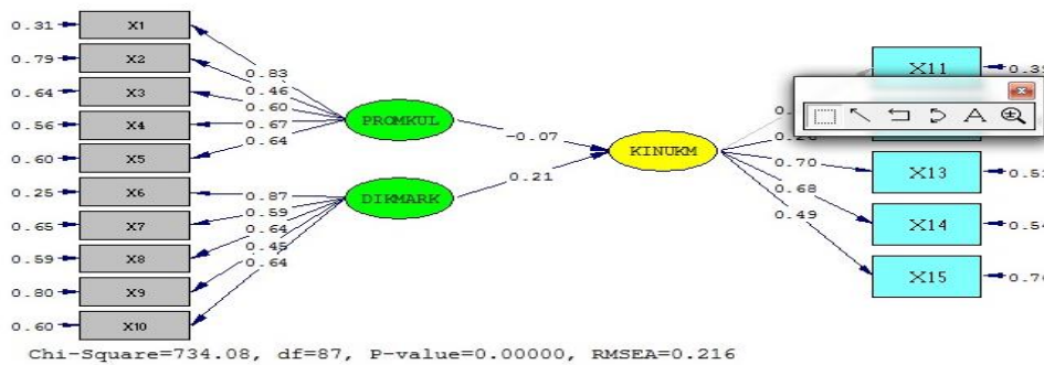
Gambar 1. Manifested Variabel
